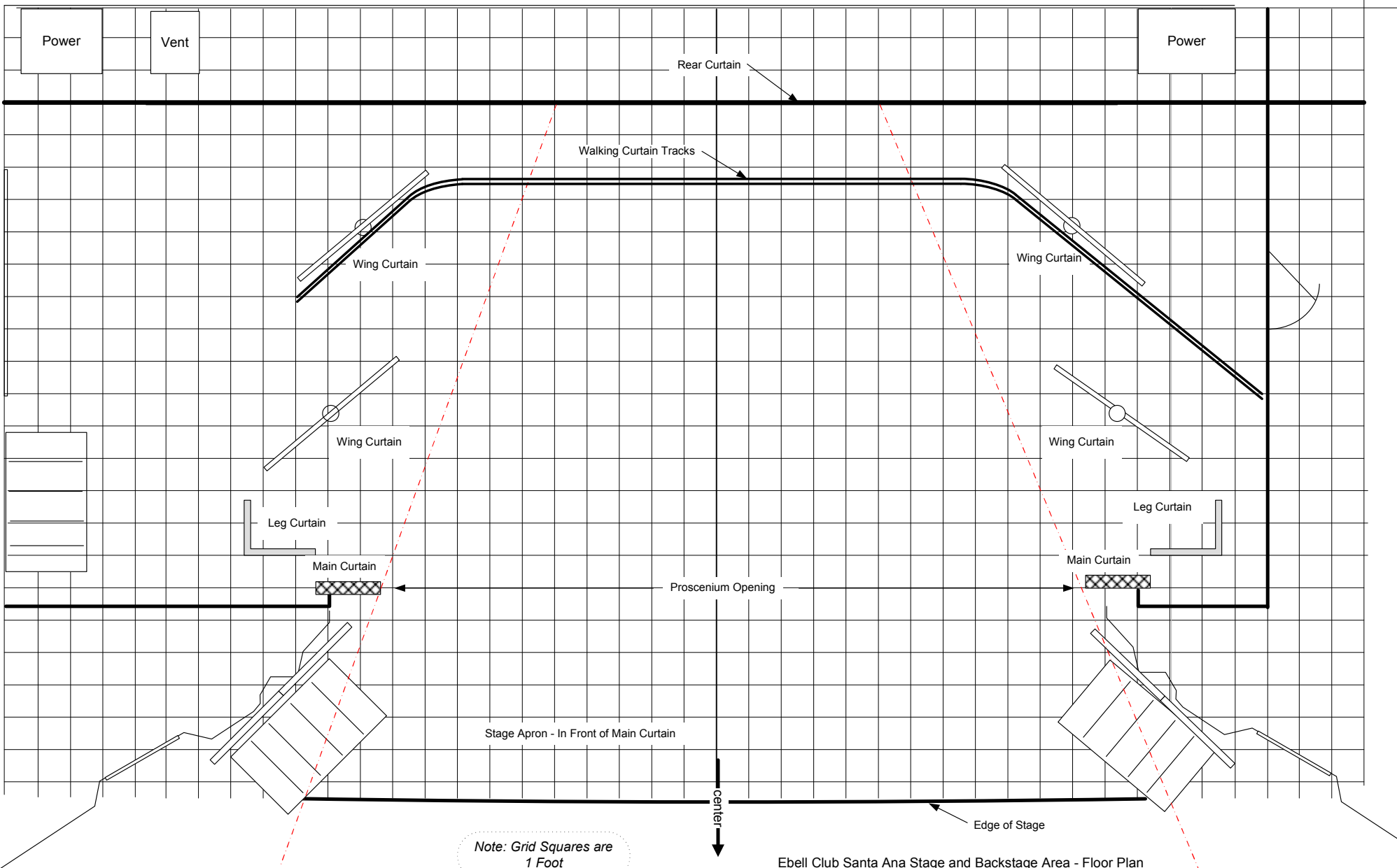
Ebelle Club Santa Ana Stage and Backstage Area - Floor Plan
